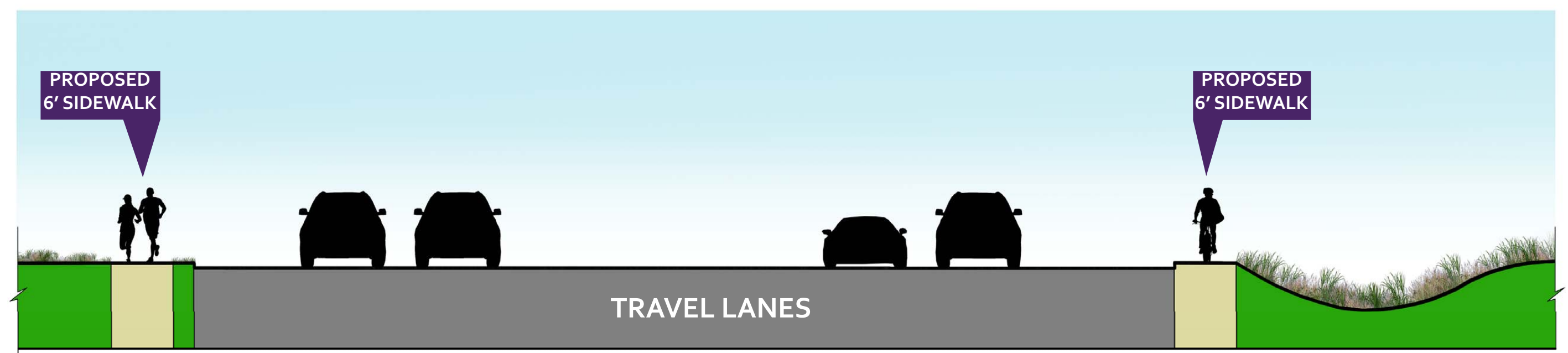
SECTION D: CLIFTY DRIVE AT MICHIGAN ROAD
