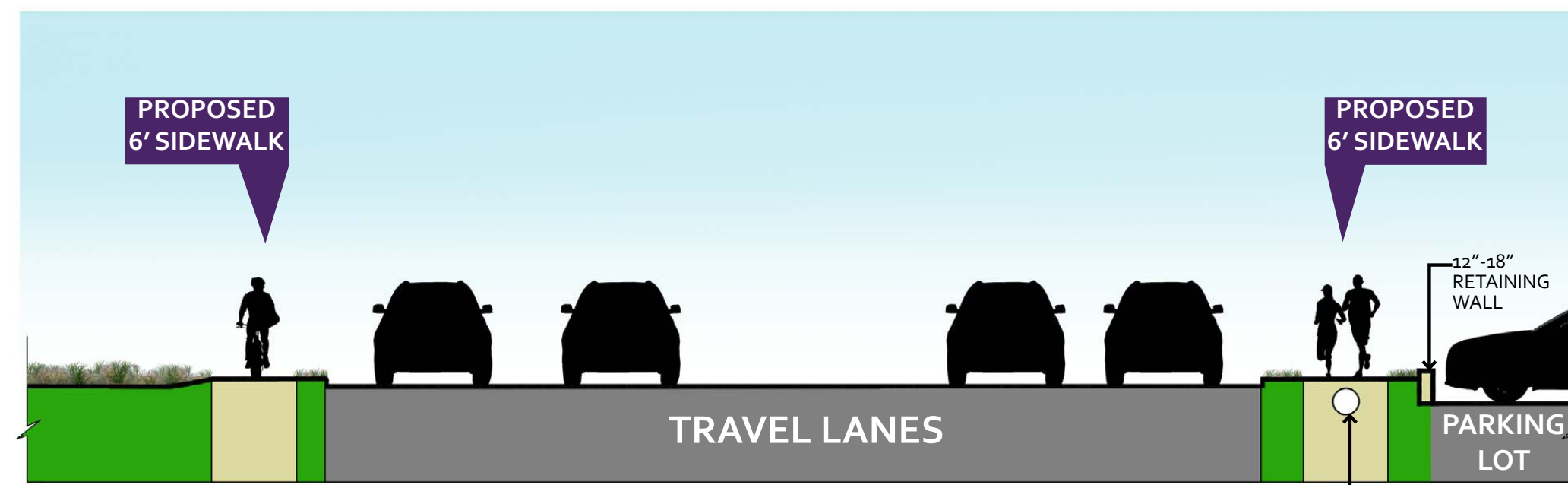
SECTION C: CLIFTY DRIVE AT CAR DEALERSHIP (TYPICAL)
